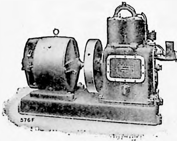
2 Crank Paraffin Engine and Dynamo.
