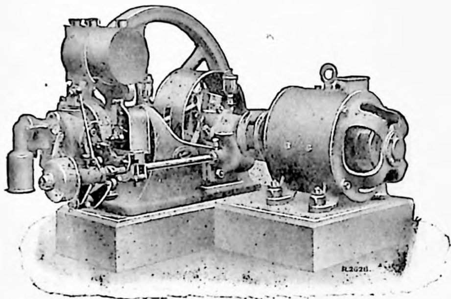
Petrol Paraffin Engine and Dynamo.
